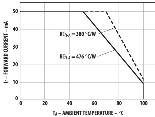
Figure 4. Maximum forward current vs. ambient temperature.
